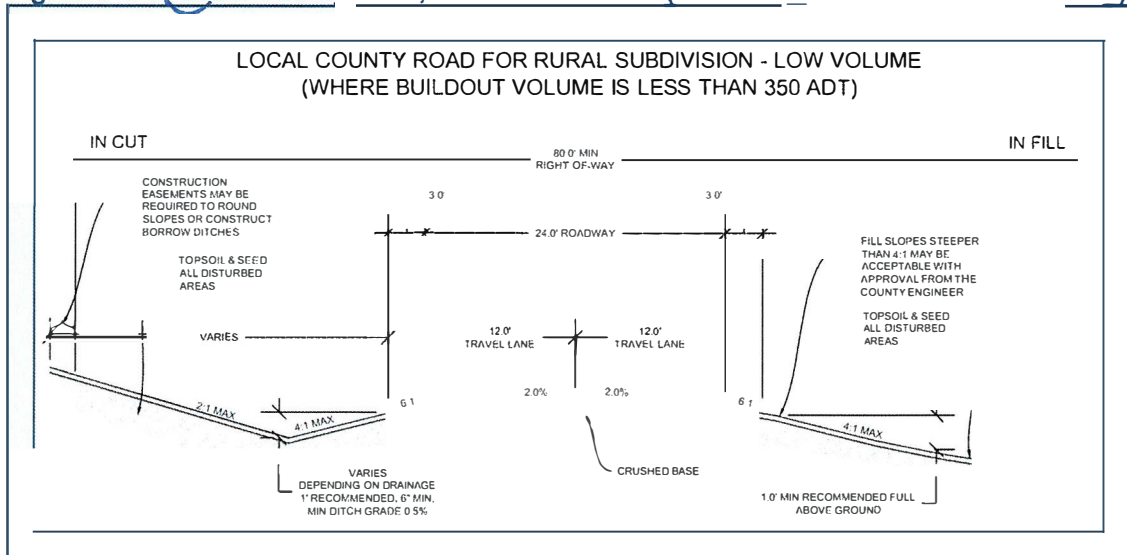
Figure 5-6-13 Local County Road, Rural Subdivision (Buildout Volume less than 350 ADT)
